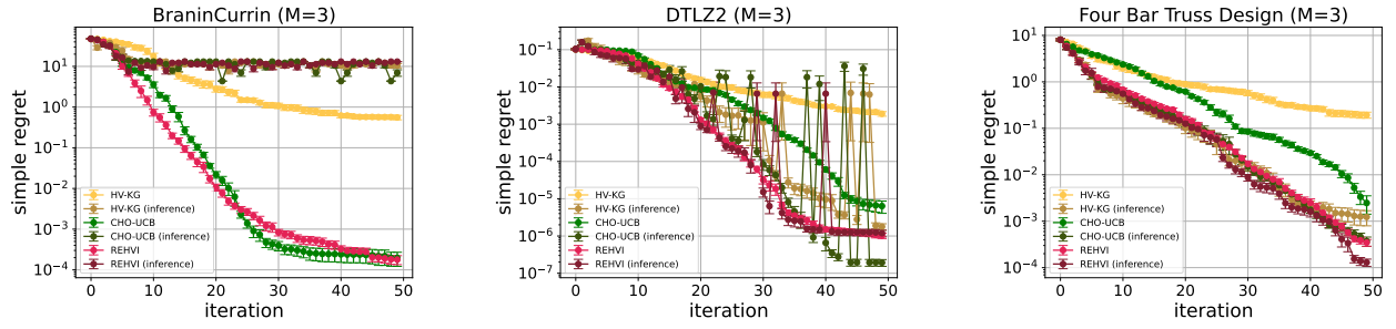
Figure 2: HVKG does not outperform the proposed methods in terms of observation regret. In terms of inference regret, all three acquisition functions perform similarly.
